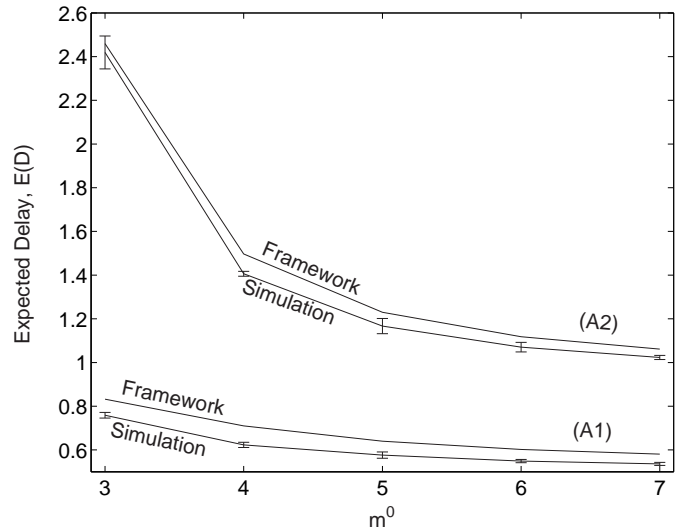
Fig. 2. Test instance (A1) and (A2). Expected B-bit delay as a function of proportionality between arrival bit rate and service bit rate.
