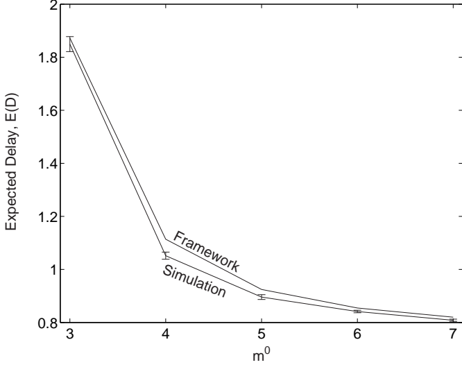
Fig. 4. Test instance (R1). Expected B-bit delay as a function of proportionality between arrival bit rate and service bit rate.
