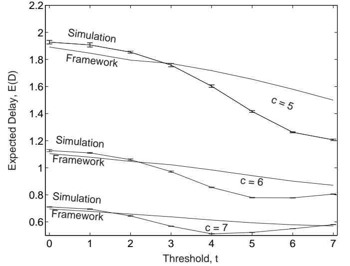
Fig. 6. Effect of varying threshold. Expected B-bit delay as a function of threshold, t . Observe the increased error margin for t \geq m^0 - 1 = 3 .
