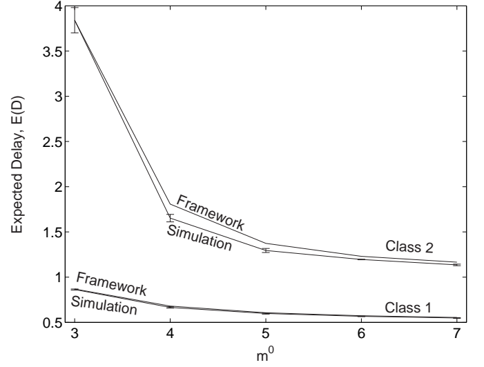
Fig. 5. Test instance (R2). Expected B-bit delay as a function of proportionality between arrival bit rate and service bit rate.
