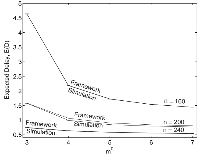
Fig. 1. Test instance (S1). Expected B-bit delay as a function of proportionality between arrival bit rate and service bit rate.
