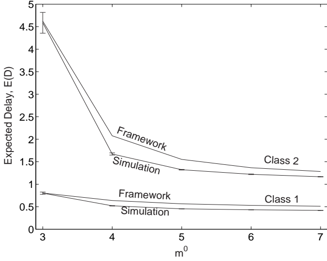
Fig. 3. Test instance (A3). Expected B-bit delay as a function of proportionality between arrival bit rate and service bit rate.
